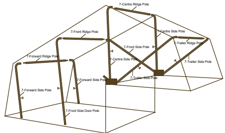
Camper Trailer Tent 7 tent poles
