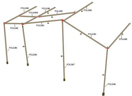
Camper Trailer Tent all 12 & 12 Twin awning poles
