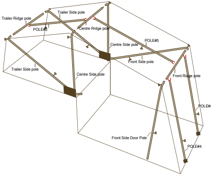
Camper Trailer Tent 8 & 8 Twin tent poles
