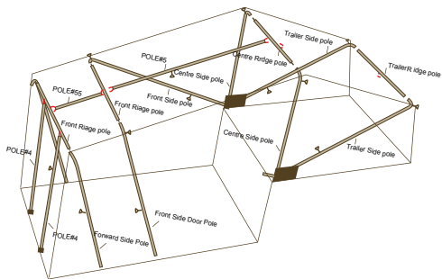
Camper Trailer Tent all 12 & 12 Twin tent poles
