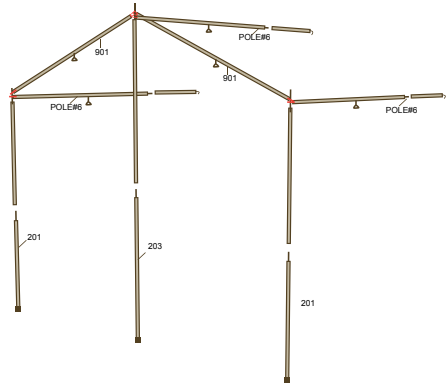
Camper Trailer Tent 6 & 7 awning poles
