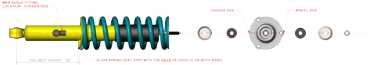
ISUZU DMAX & HOLDEN COLORADO (RG) RIGHT HAND STRUT SHOWN
