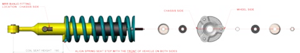
MAZDA BT50 & FORD RANGER (PX) LEFT HAND STRUT SHOWN
