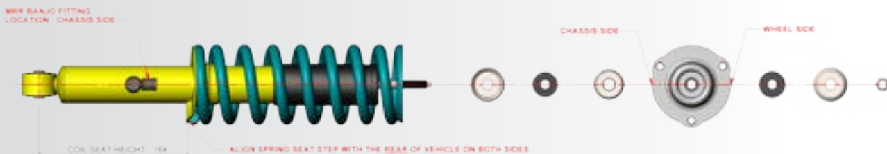
TOYOTA LANDCRUISER (PRADO 90) RIGHT HAND STRUT SHOWN
